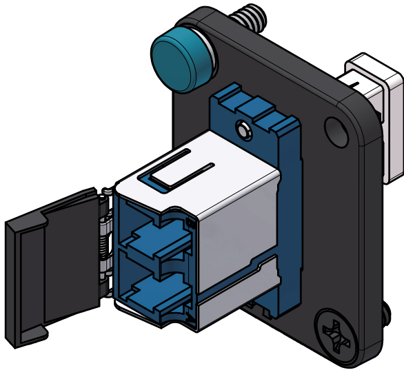
UMF-SMD-LC-BL-SH kit shown with the Shutter Door open
